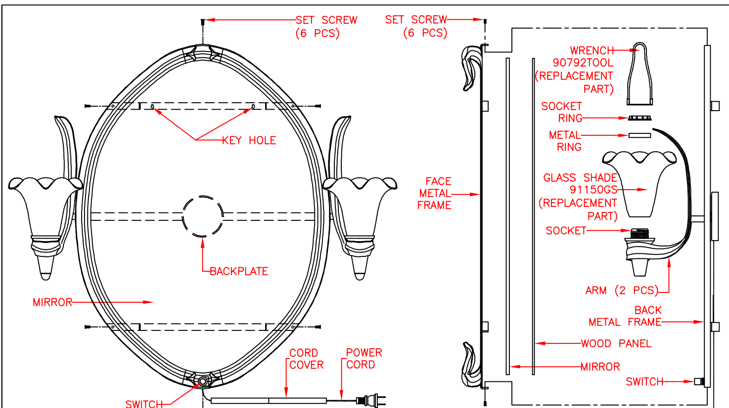
SIDE VIEW
